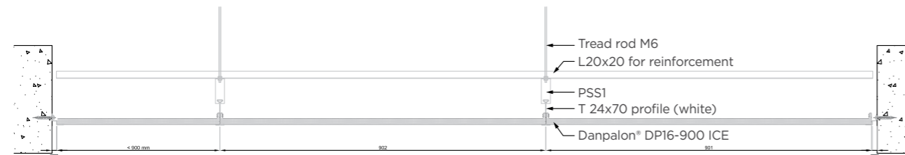
Cut A-A: on reinforcement area
